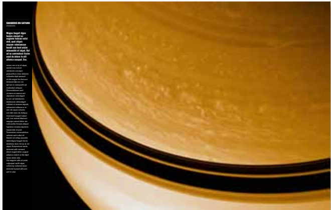
PLANETS
