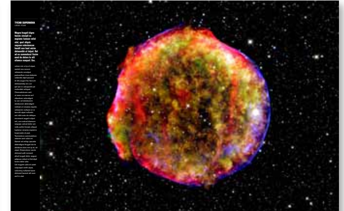
SUPERNOVA
